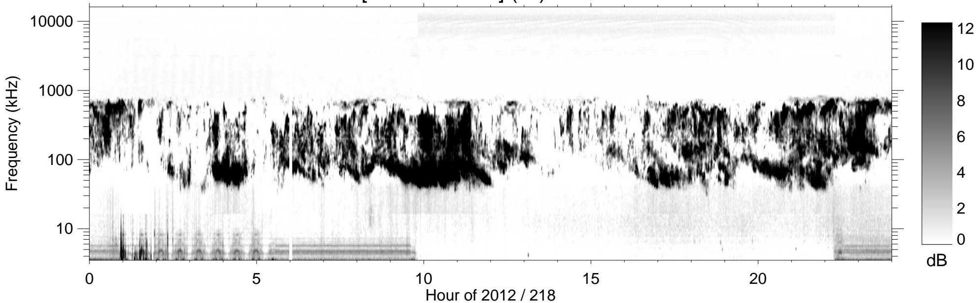
RPWS [ABCH1H2/Ex] (-B) 2012/08/05
