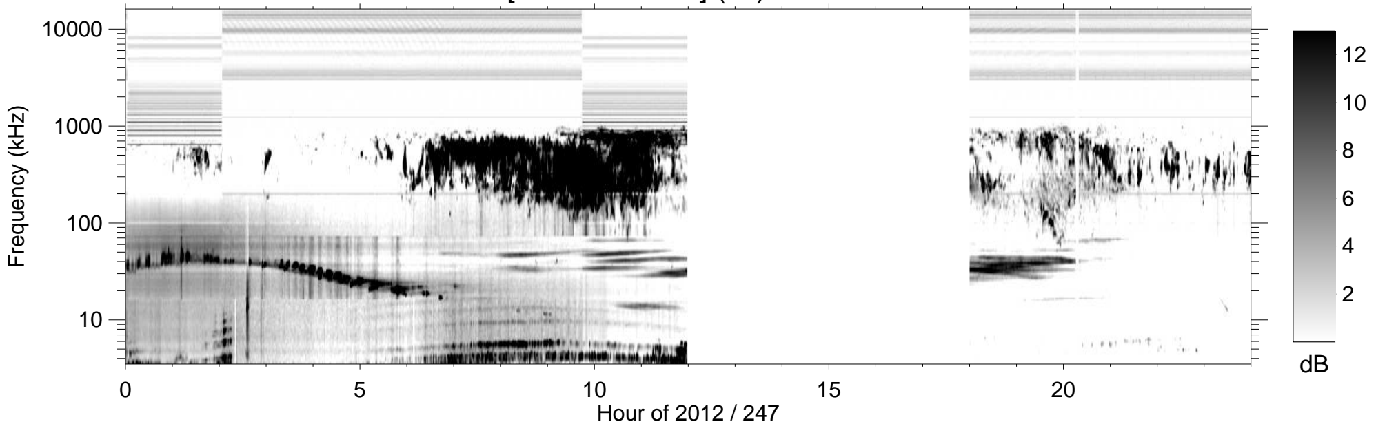
RPWS [ABCH1H2/Ex] (-B) 2012/09/03
