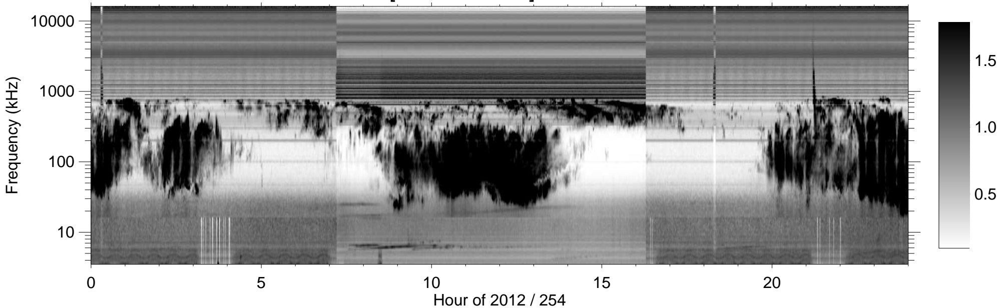
RPWS [ABCH1H2/Ex] (-B) 2012/09/10
