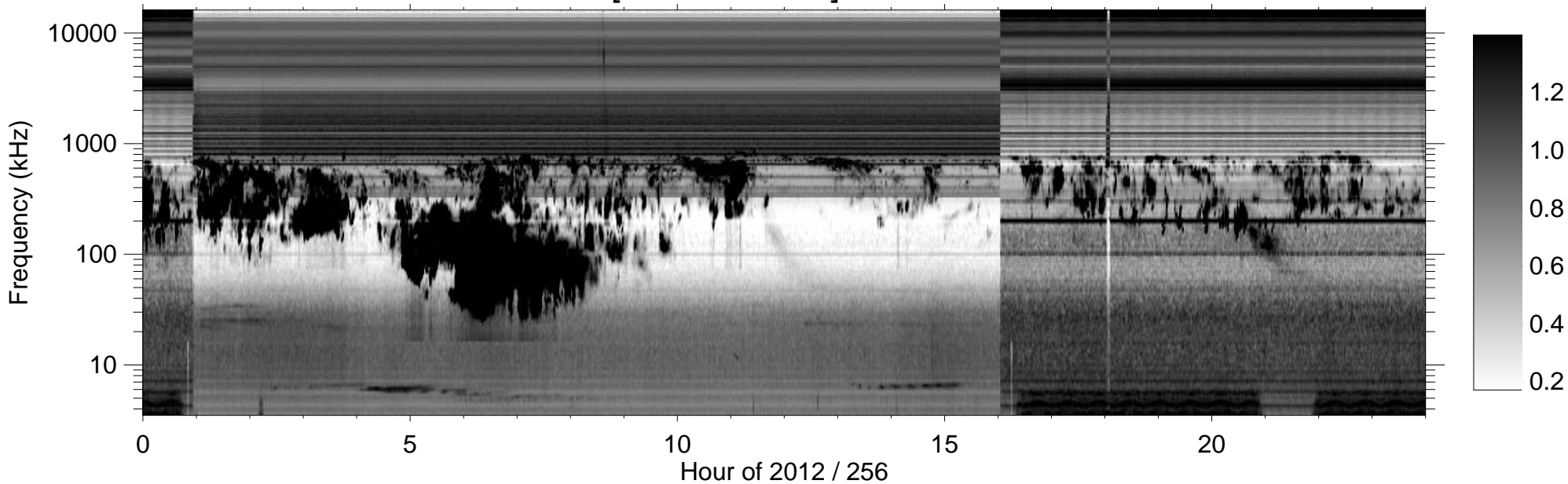
RPWS [ABCH1H2/Ex] (-B) 2012/09/12
