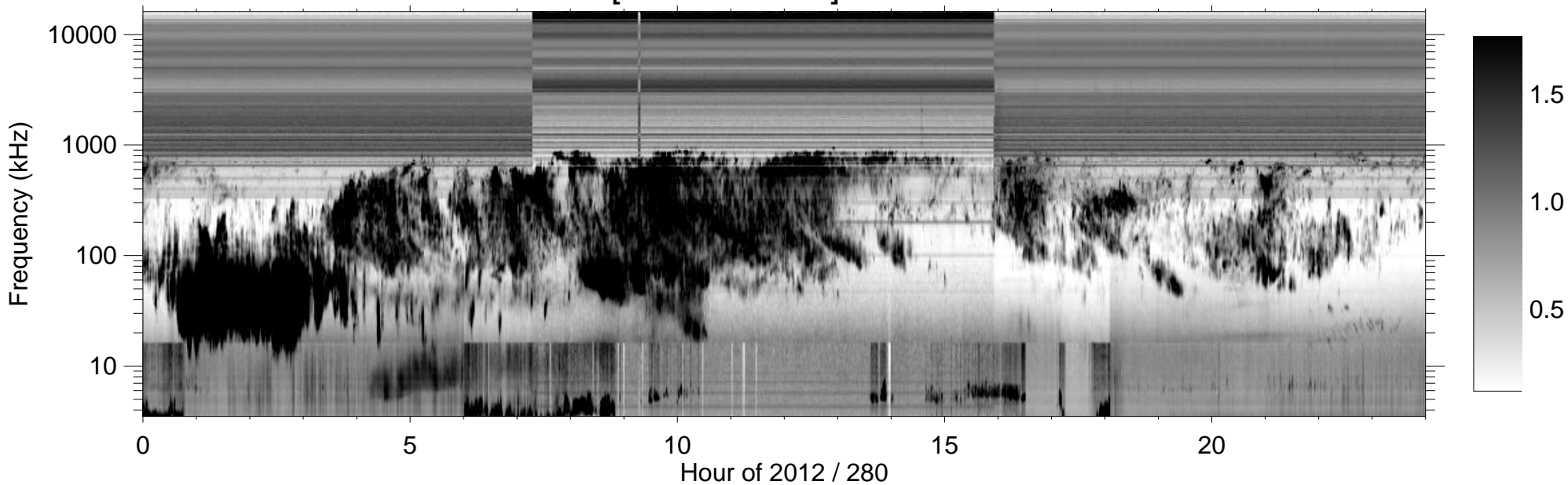
RPWS [ABCH1H2/Ex] (-B) 2012/10/06
