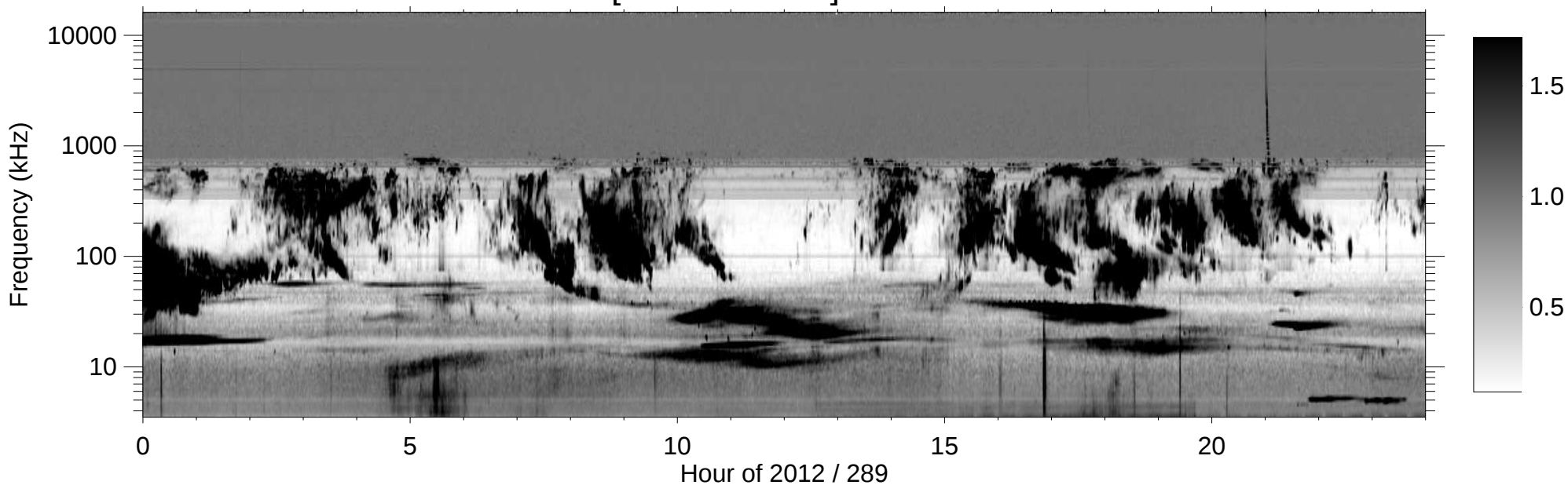
RPWS [ABCH1H2/Ex] (-B) 2012/10/15
