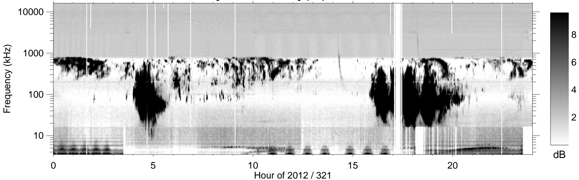
RPWS [ABCH1H2/Ex] (-B) 2012/11/16
