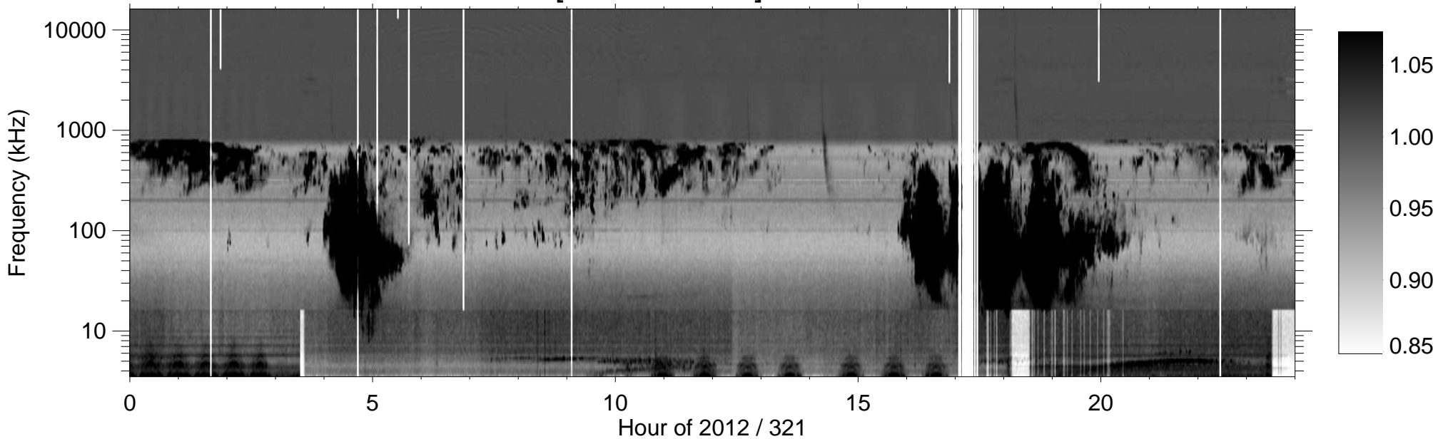
RPWS [ABCH1H2/Ex] (-B) 2012/11/16
