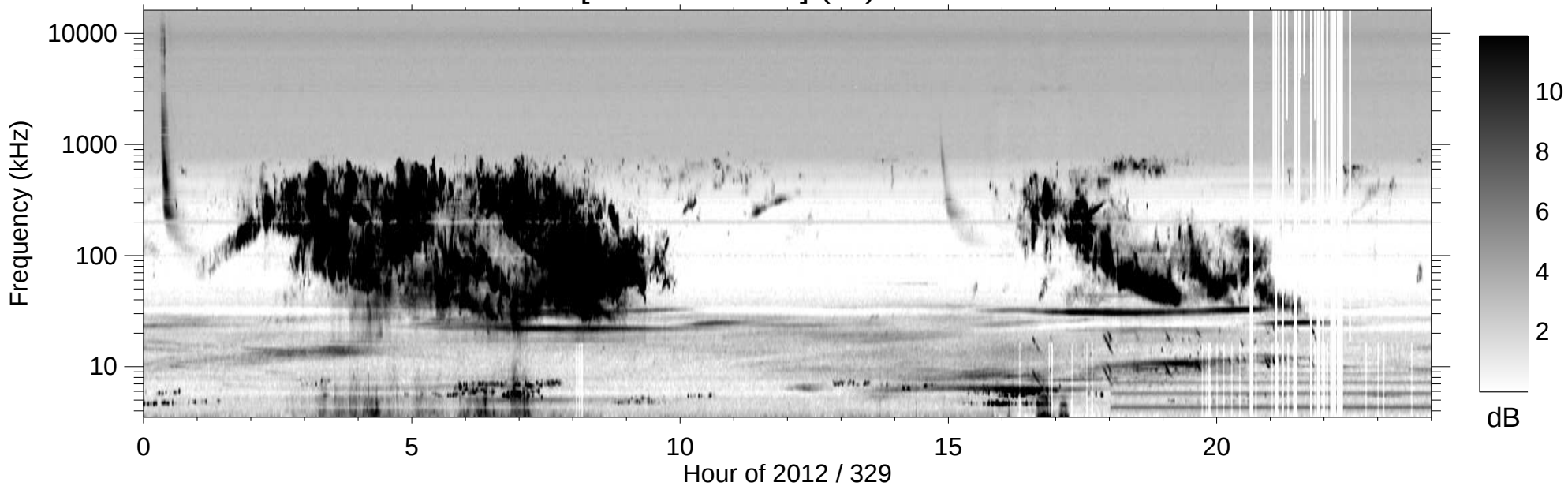
RPWS [ABCH1H2/Ex] (-B) 2012/11/24
