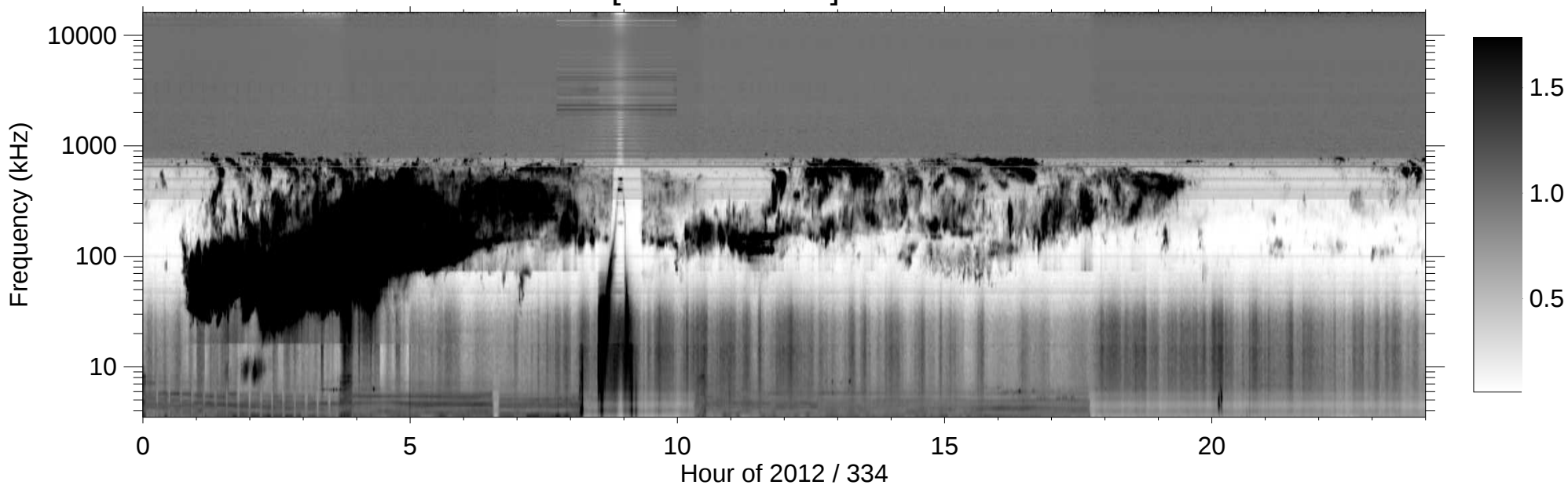
RPWS [ABCH1H2/Ex] (-B) 2012/11/29
