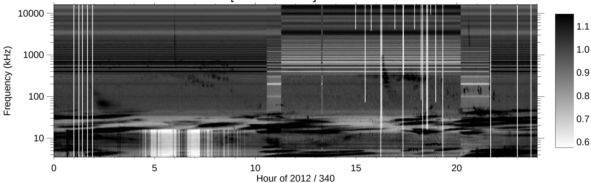
RPWS [ABCH1H2/Ex] (-B) 2012/12/05
