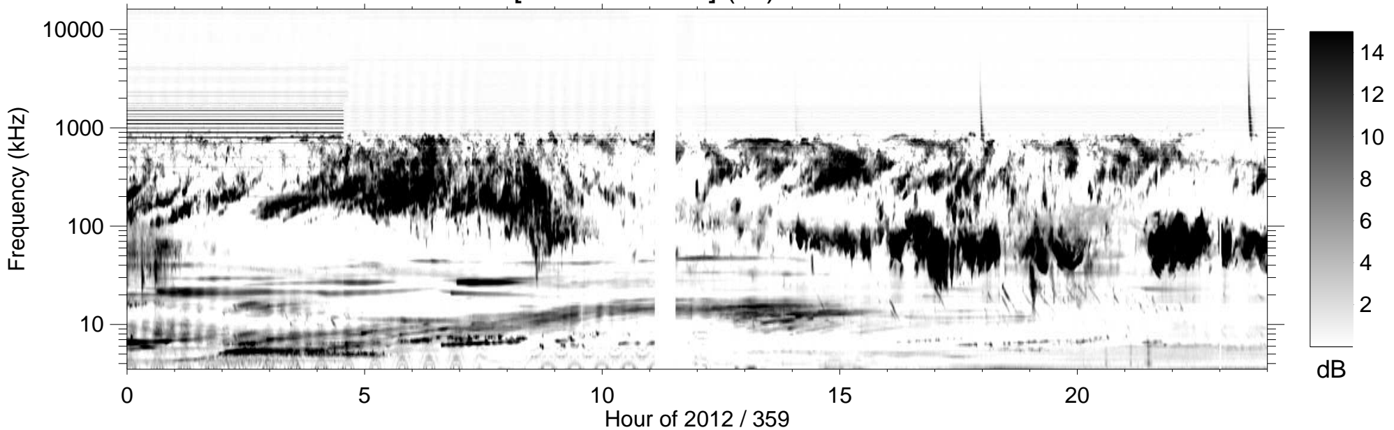
RPWS [ABCH1H2/Ex] (-B) 2012/12/24
