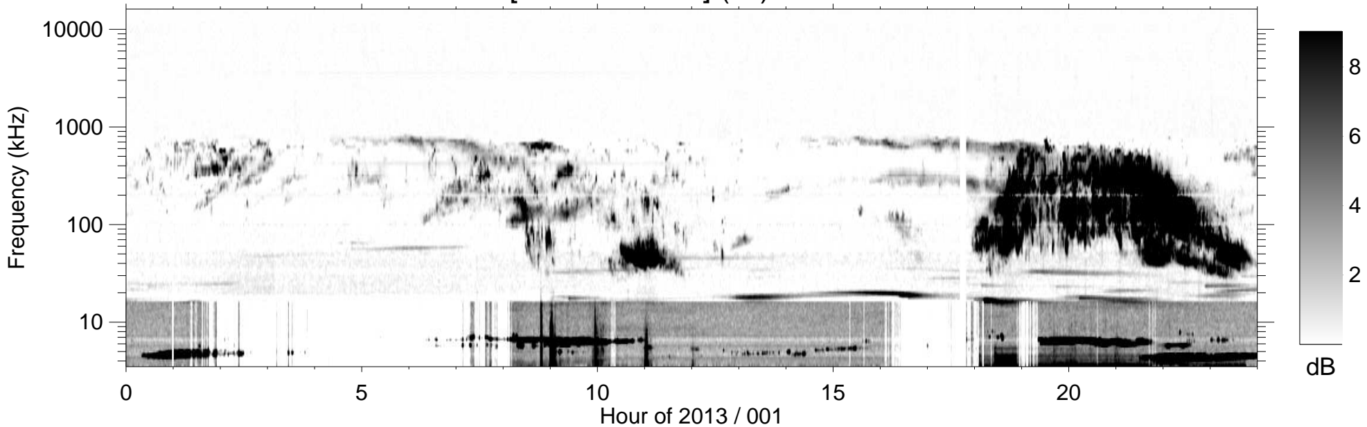
RPWS [ABCH1H2/Ex] (-B) 2013/01/01
