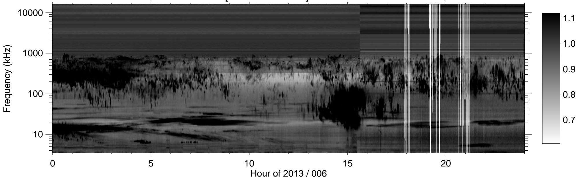
RPWS [ABCH1H2/Ex] (-B) 2013/01/06
