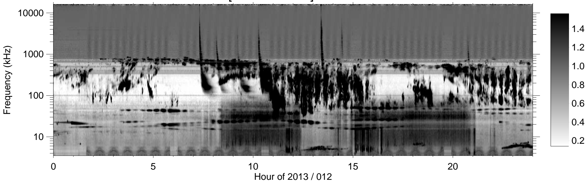
RPWS [ABCH1H2/Ex] (-B) 2013/01/12
