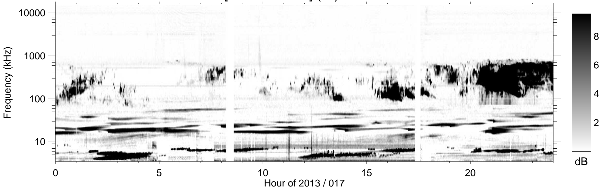
RPWS [ABCH1H2/Ex] (-B) 2013/01/17
