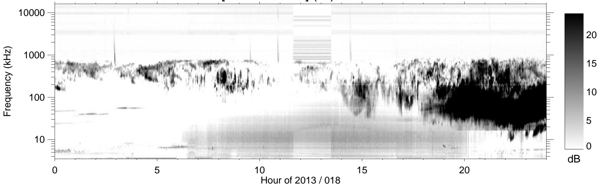
RPWS [ABCH1H2/Ex] (-B) 2013/01/18
