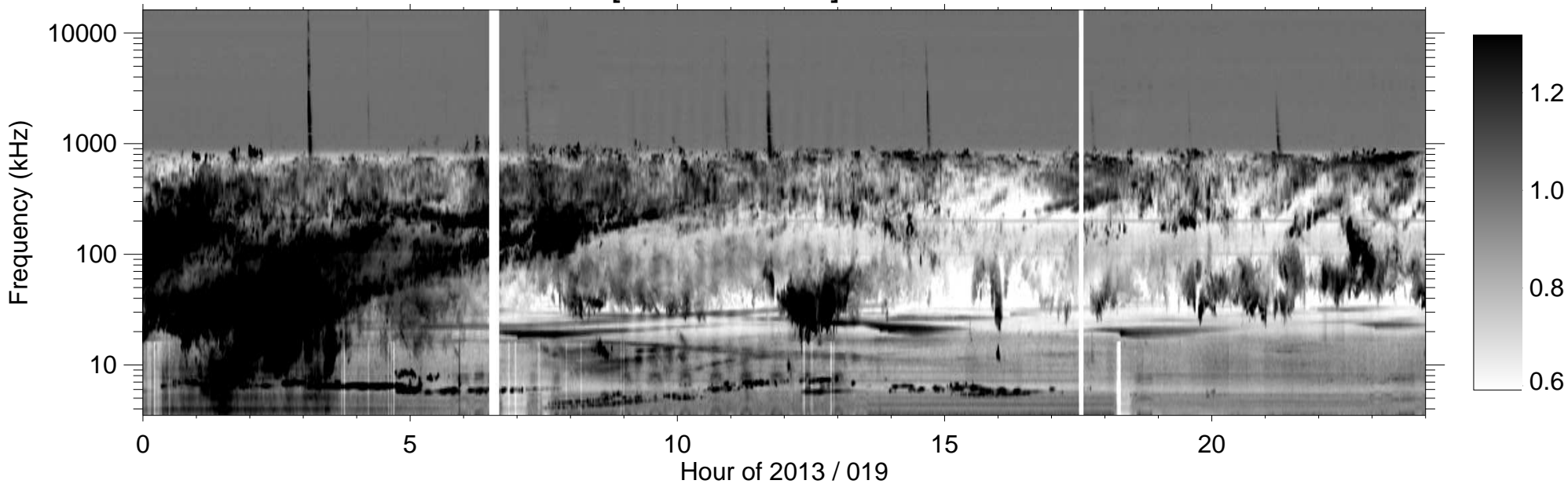
RPWS [ABCH1H2/Ex] (-B) 2013/01/19
