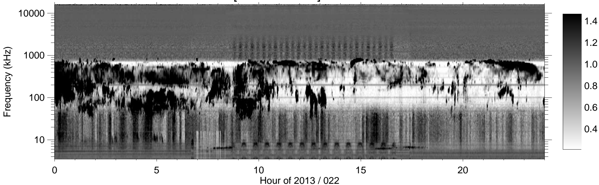
RPWS [ABCH1H2/Ex] (-B) 2013/01/22
