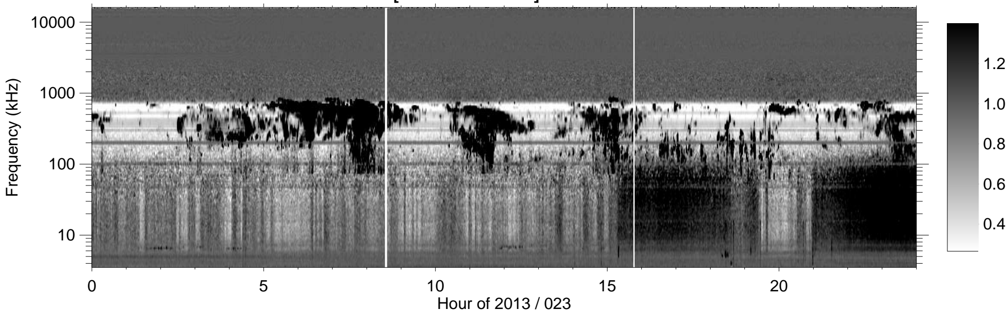
RPWS [ABCH1H2/Ex] (-B) 2013/01/23
