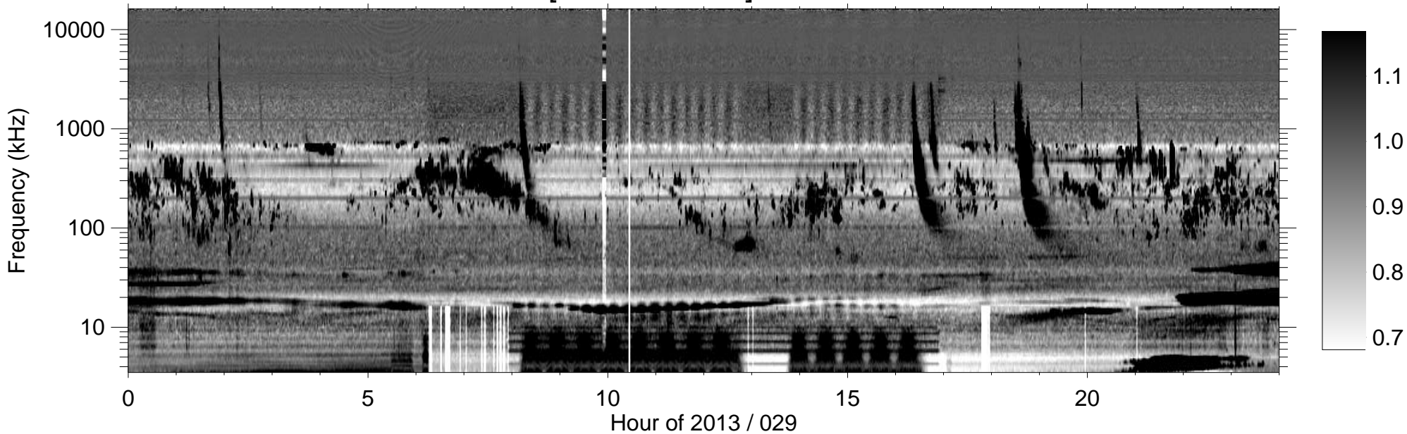
RPWS [ABCH1H2/Ex] (-B) 2013/01/29
