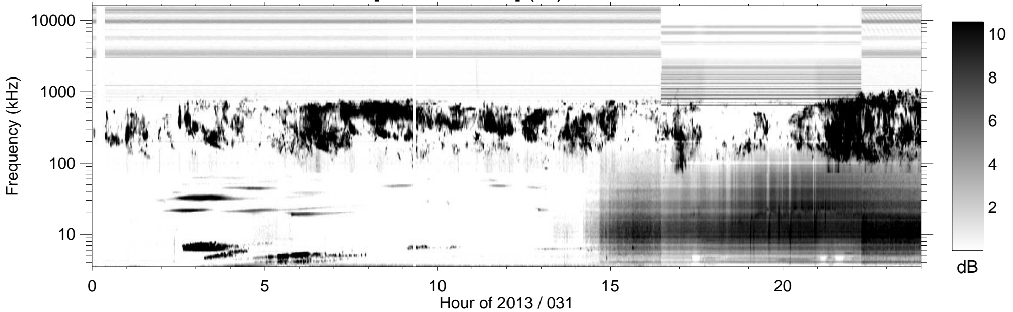
RPWS [ABCH1H2/Ex] (-B) 2013/01/31
