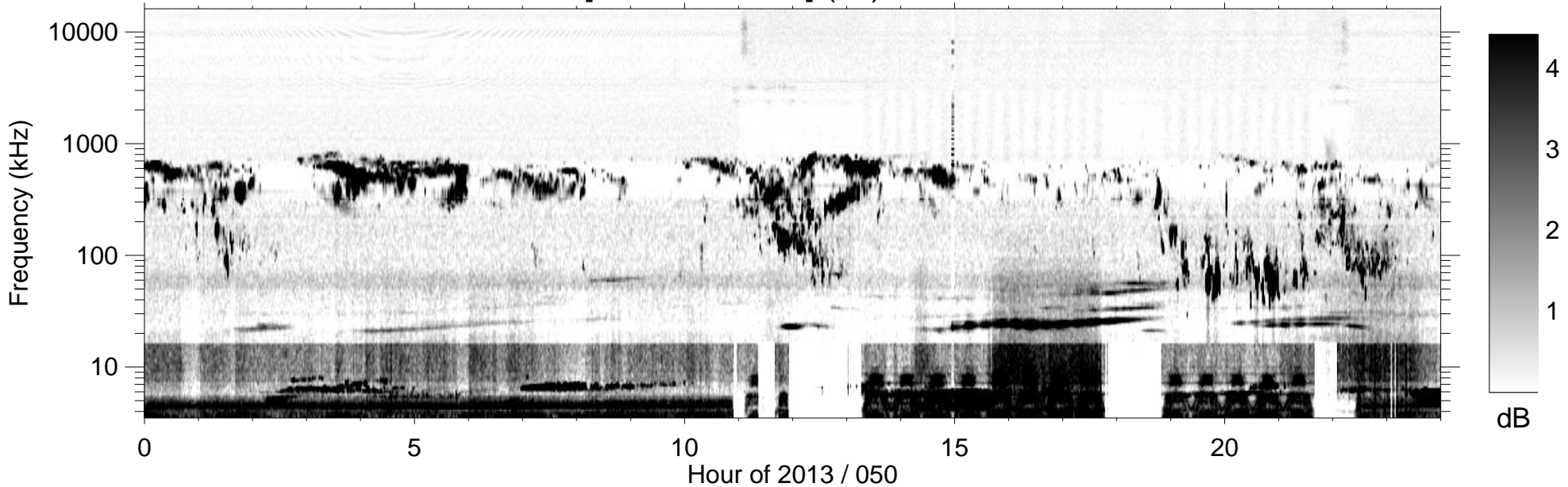
RPWS [ABCH1H2/Ex] (-B) 2013/02/19
