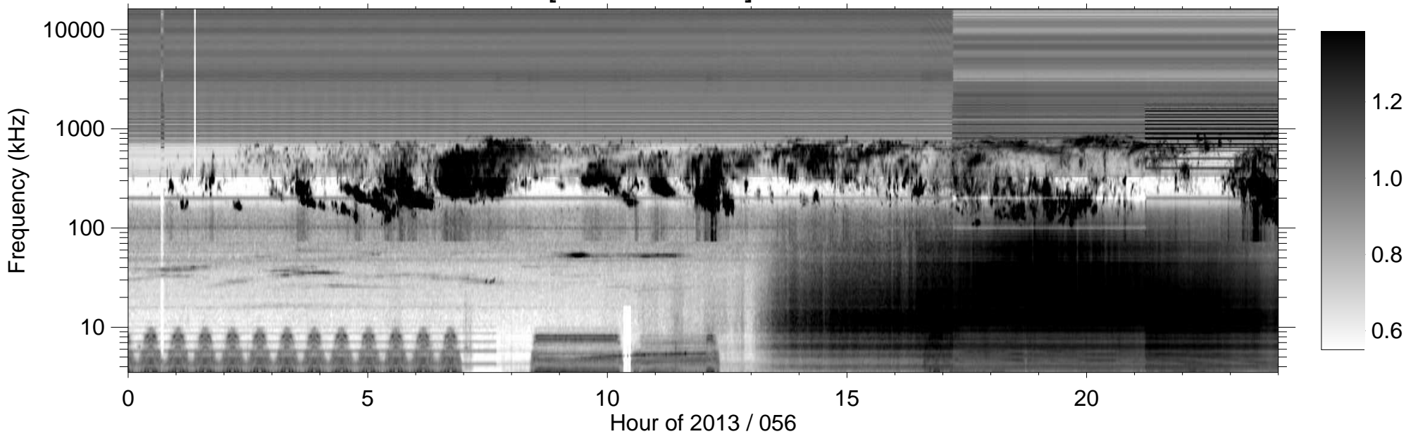
RPWS [ABCH1H2/Ex] (-B) 2013/02/25
