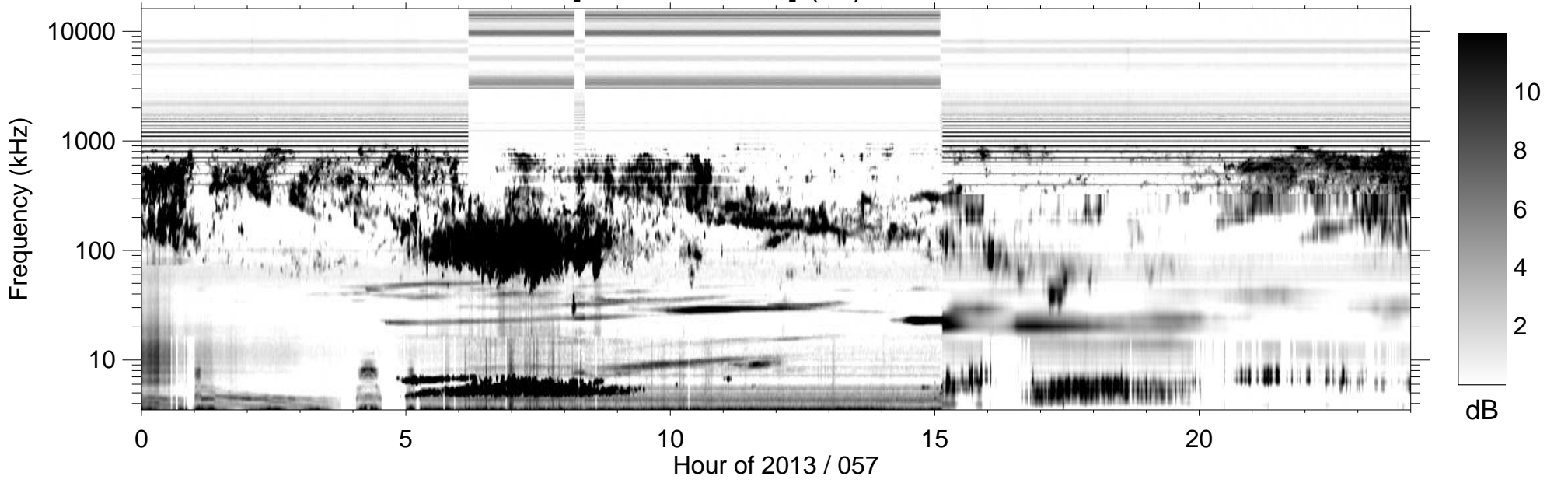
RPWS [ABCH1H2/Ex] (-B) 2013/02/26
