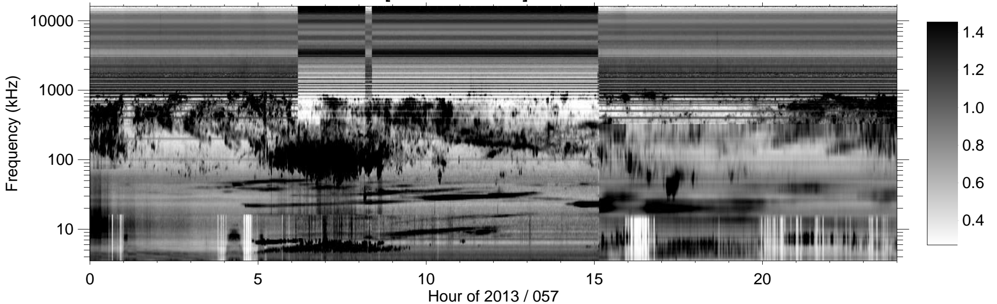
RPWS [ABCH1H2/Ex] (-B) 2013/02/26
