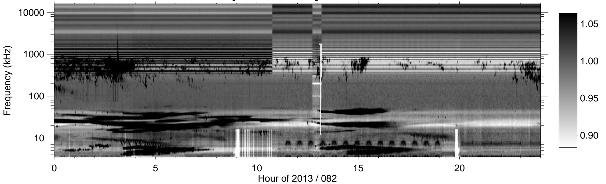
RPWS [ABCH1H2/Ex] (-B) 2013/03/23
