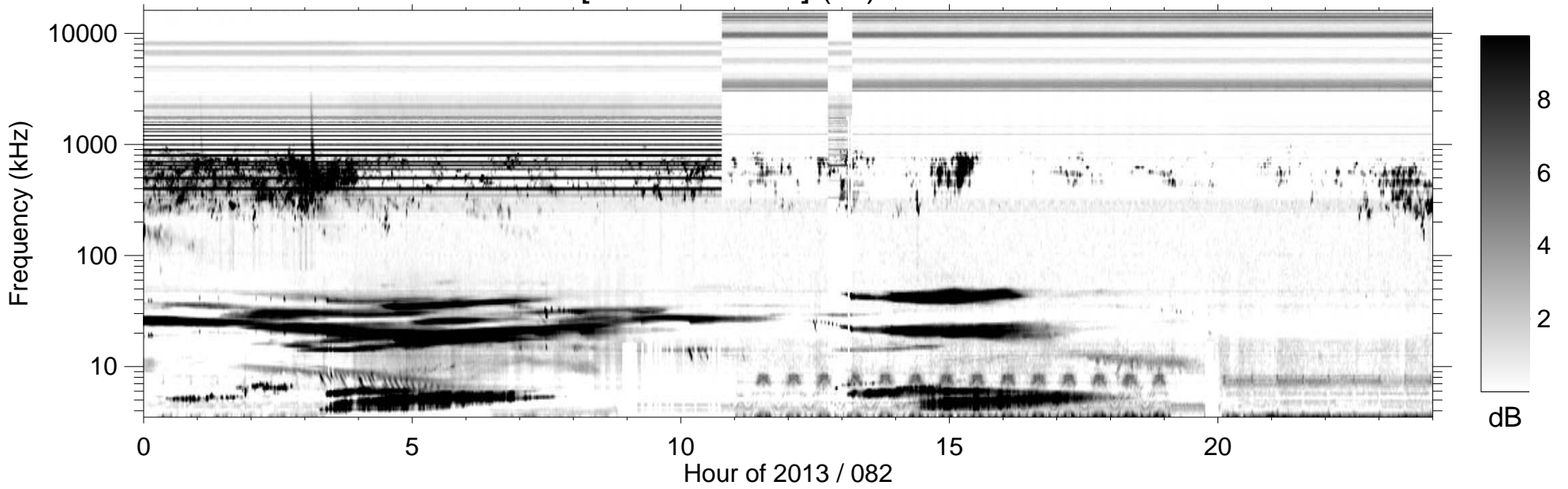
RPWS [ABCH1H2/Ex] (-B) 2013/03/23
