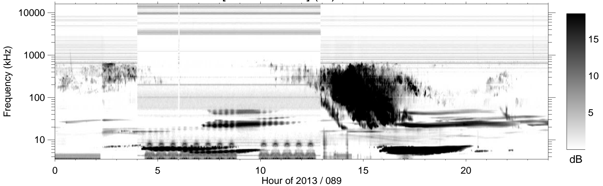
RPWS [ABCH1H2/Ex] (-B) 2013/03/30
