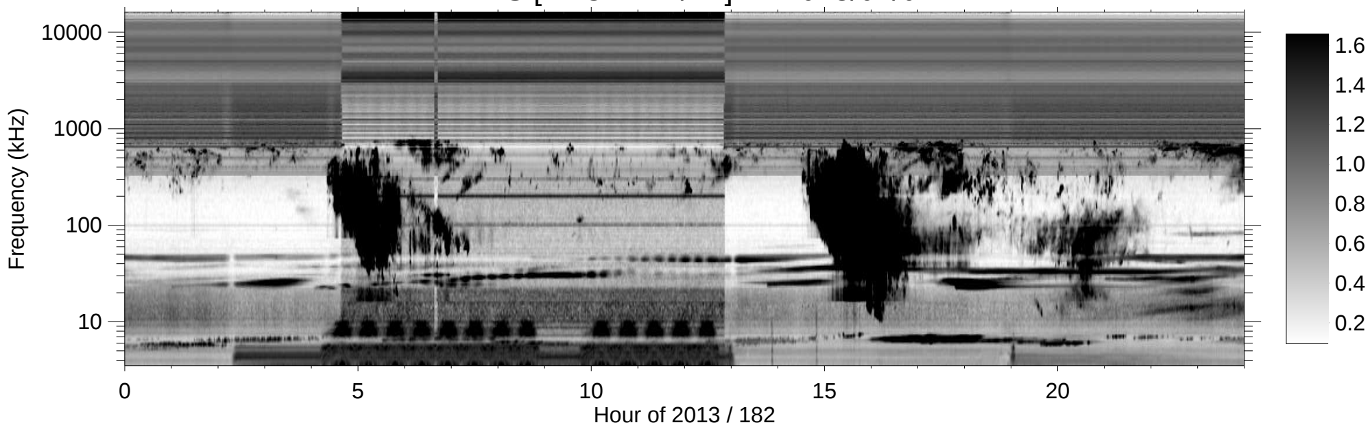
RPWS [ABCH1H2/Ex] (-B) 2013/07/01
