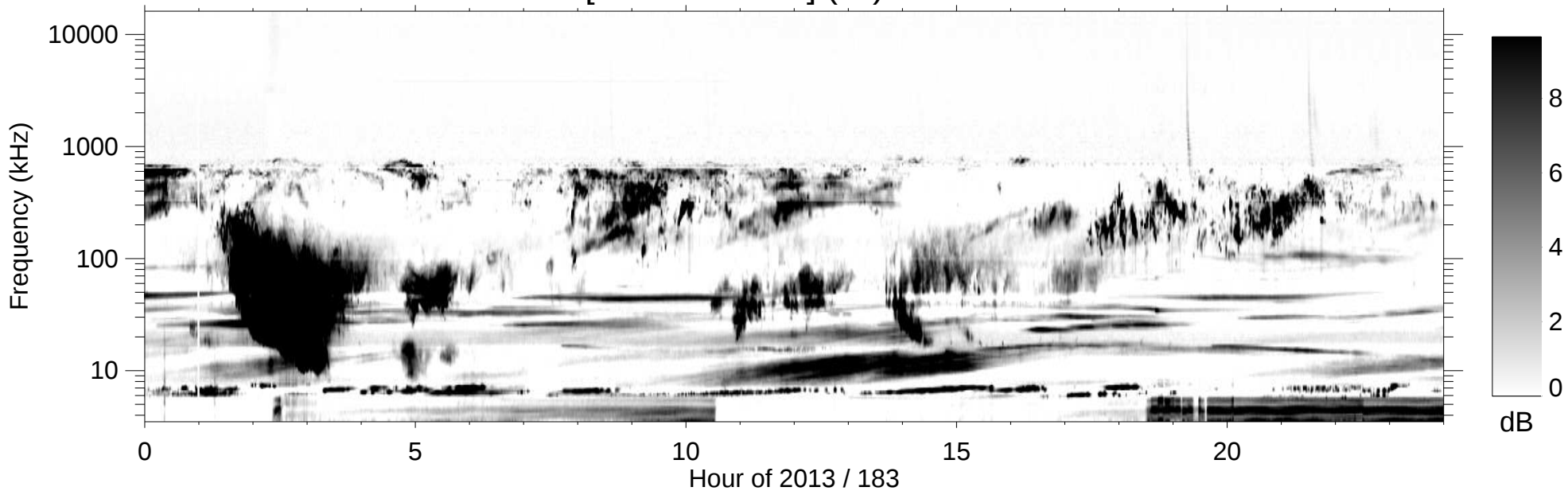
RPWS [ABCH1H2/Ex] (-B) 2013/07/02
