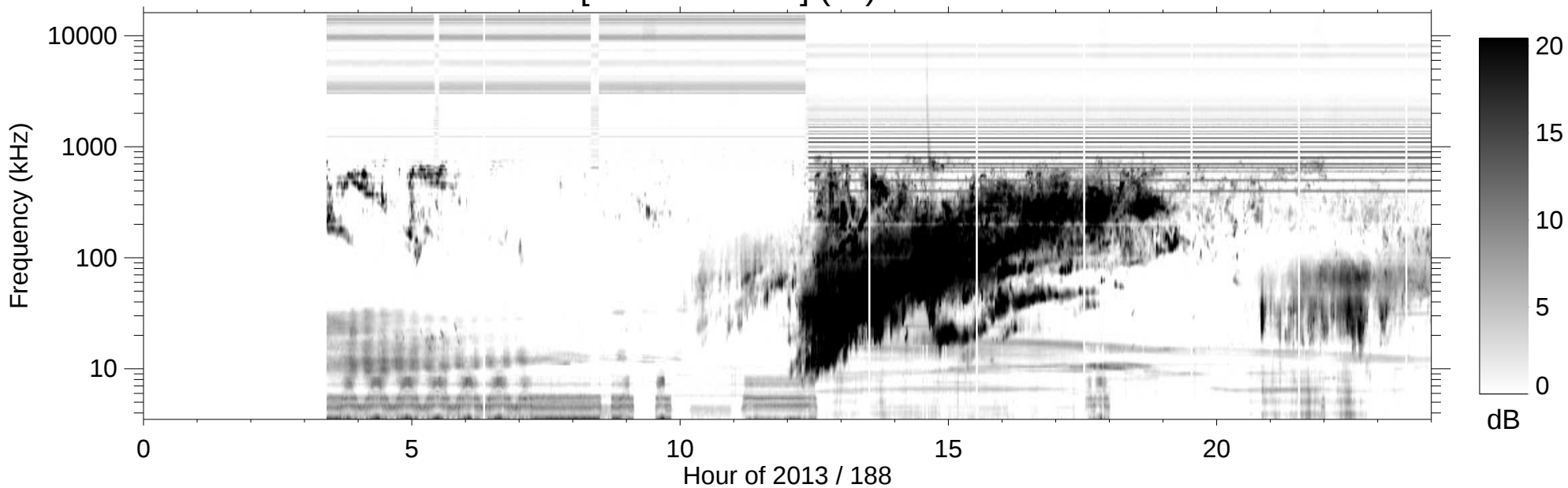
RPWS [ABCH1H2/Ex] (-B) 2013/07/07
