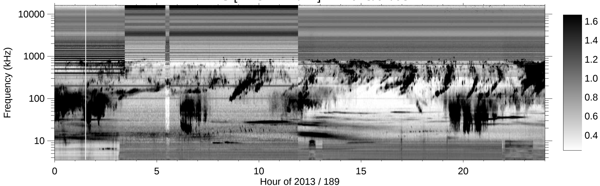
RPWS [ABCH1H2/Ex] (-B) 2013/07/08
