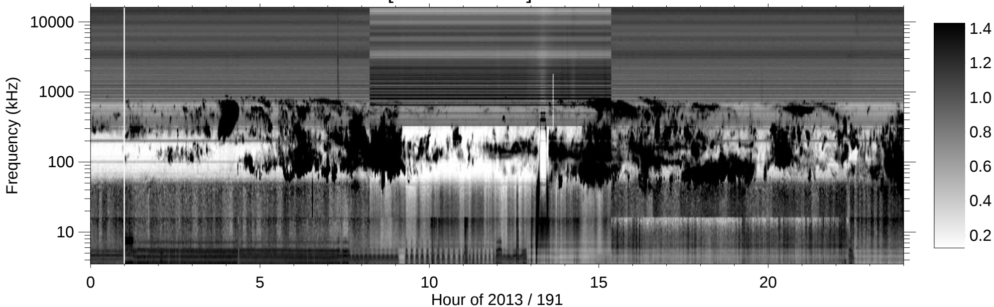
RPWS [ABCH1H2/Ex] (-B) 2013/07/10
