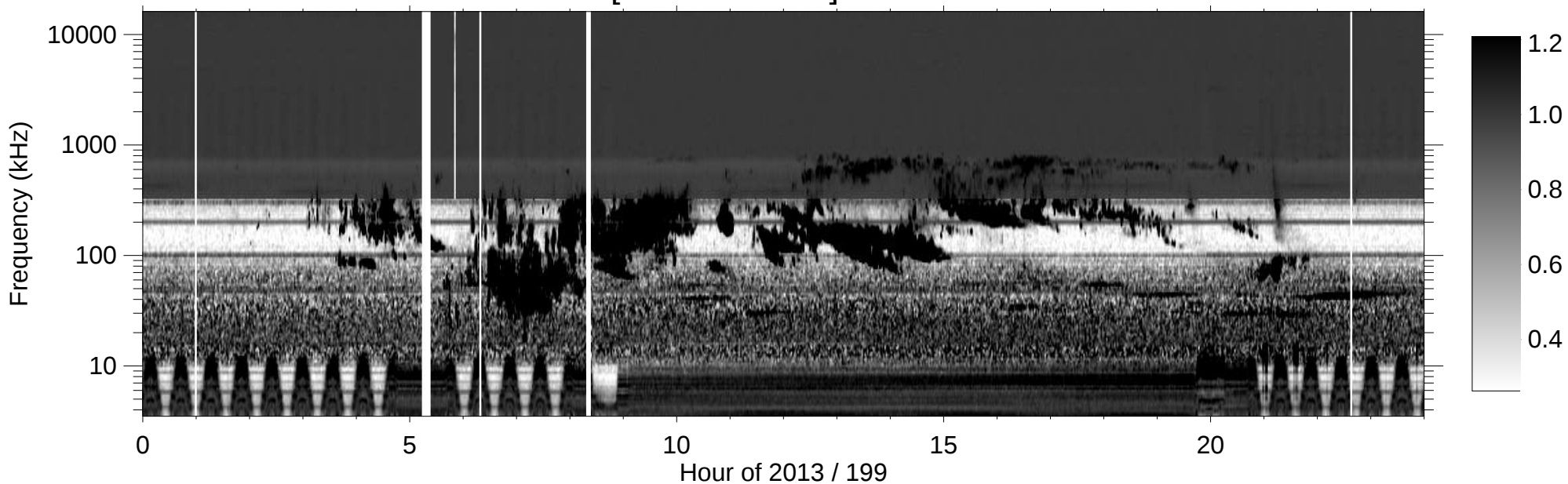
RPWS [ABCH1H2/Ex] (-B) 2013/07/18
