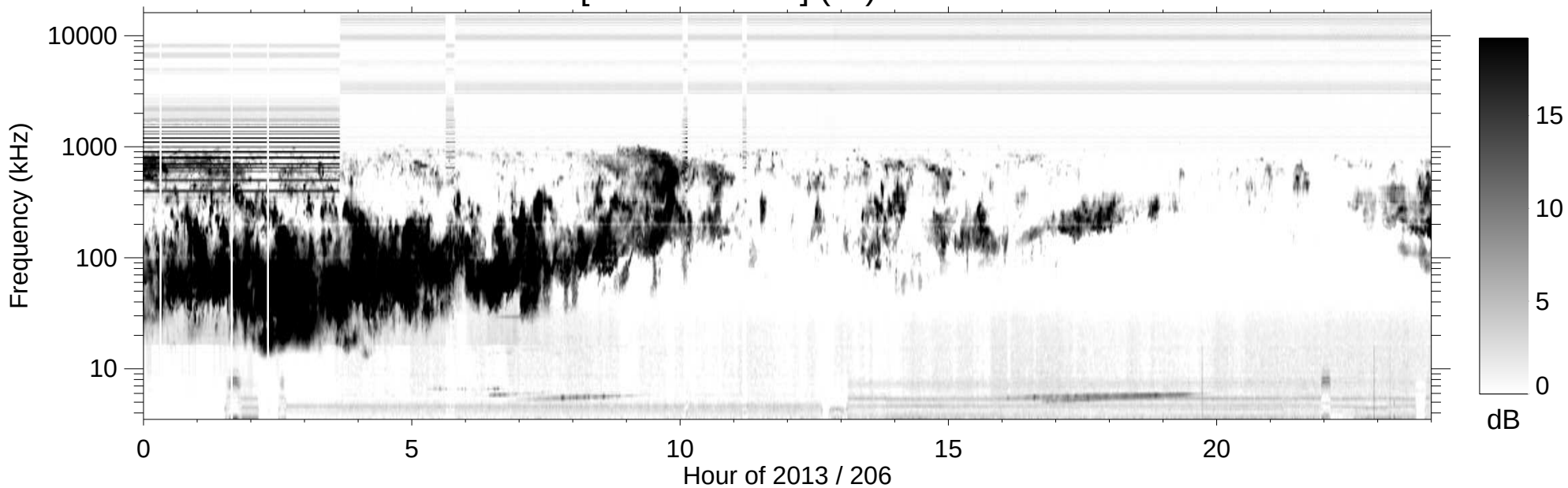
RPWS [ABCH1H2/Ex] (-B) 2013/07/25
