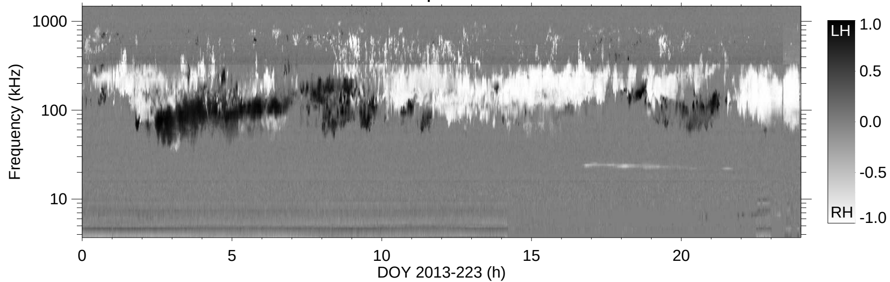
Circular polarization
