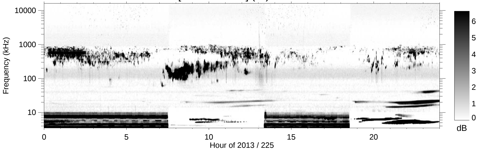
RPWS [ABCH1H2/Ex] (-B) 2013/08/13
