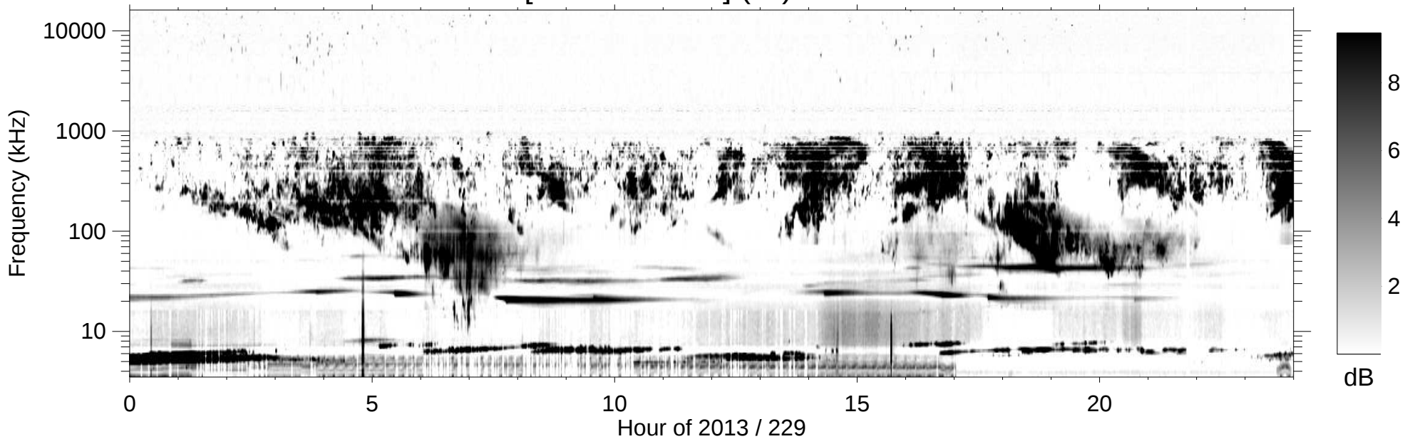
RPWS [ABCH1H2/Ex] (-B) 2013/08/17
