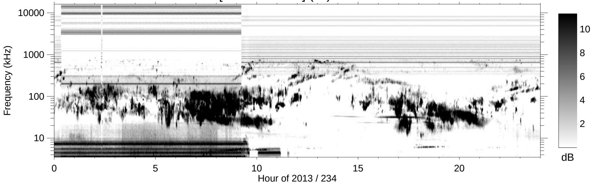
RPWS [ABCH1H2/Ex] (-B) 2013/08/22
