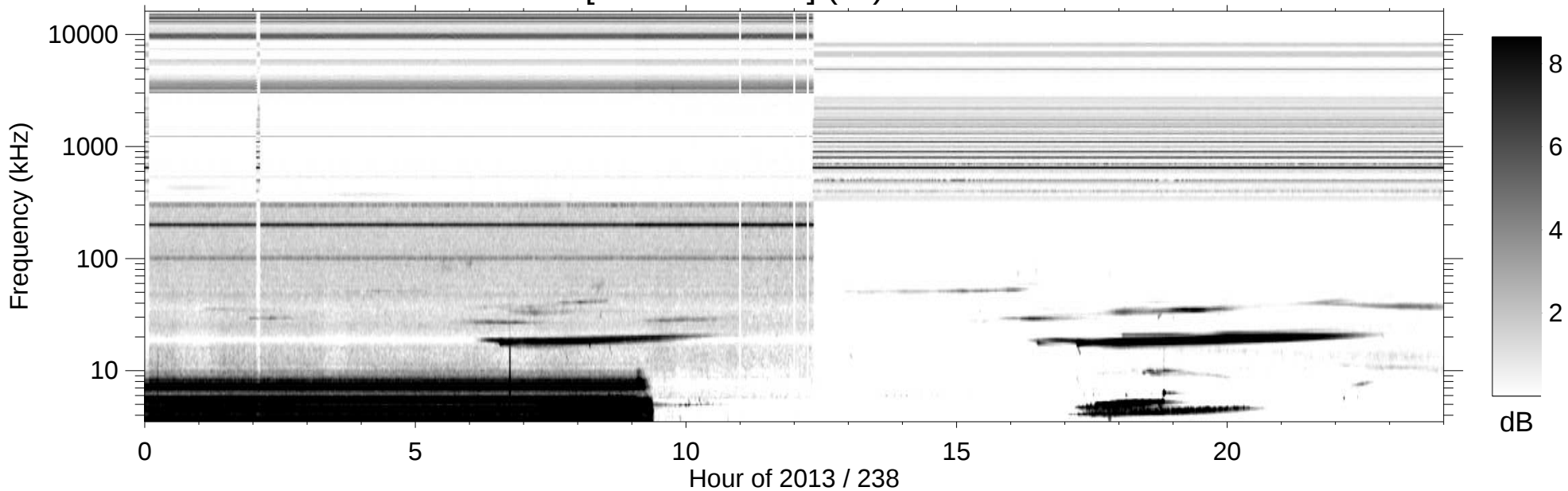
RPWS [ABCH1H2/Ex] (-B) 2013/08/26
