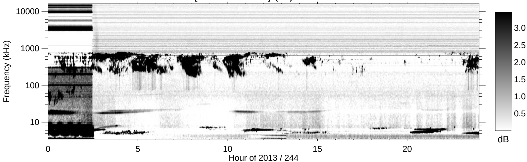
RPWS [ABCH1H2/Ex] (-B) 2013/09/01
