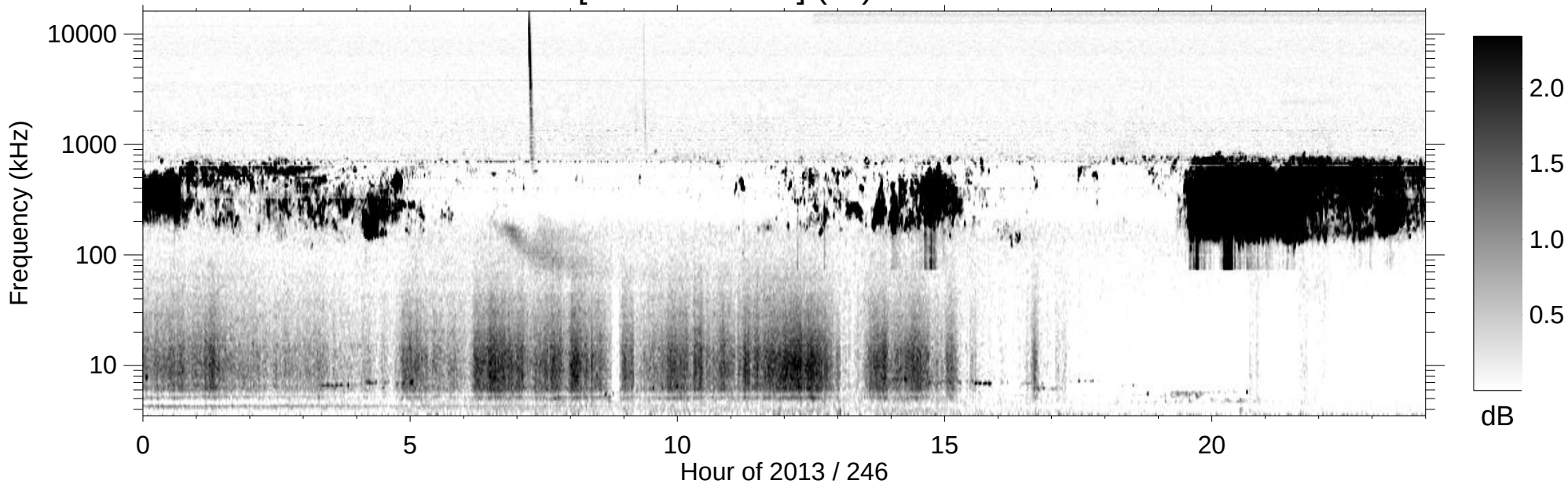
RPWS [ABCH1H2/Ex] (-B) 2013/09/03
