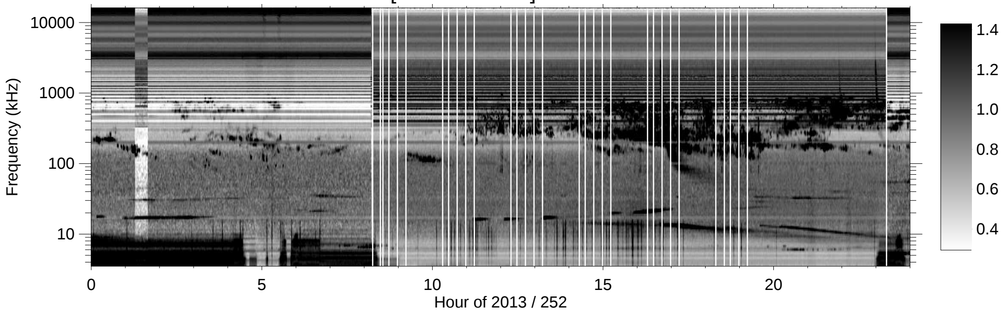
RPWS [ABCH1H2/Ex] (-B) 2013/09/09
