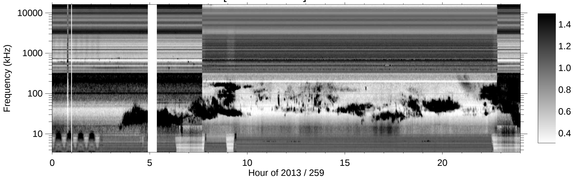
RPWS [ABCH1H2/Ex] (-B) 2013/09/16
