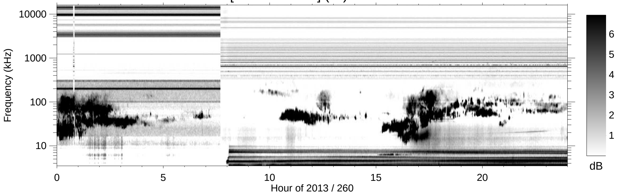
RPWS [ABCH1H2/Ex] (-B) 2013/09/17
