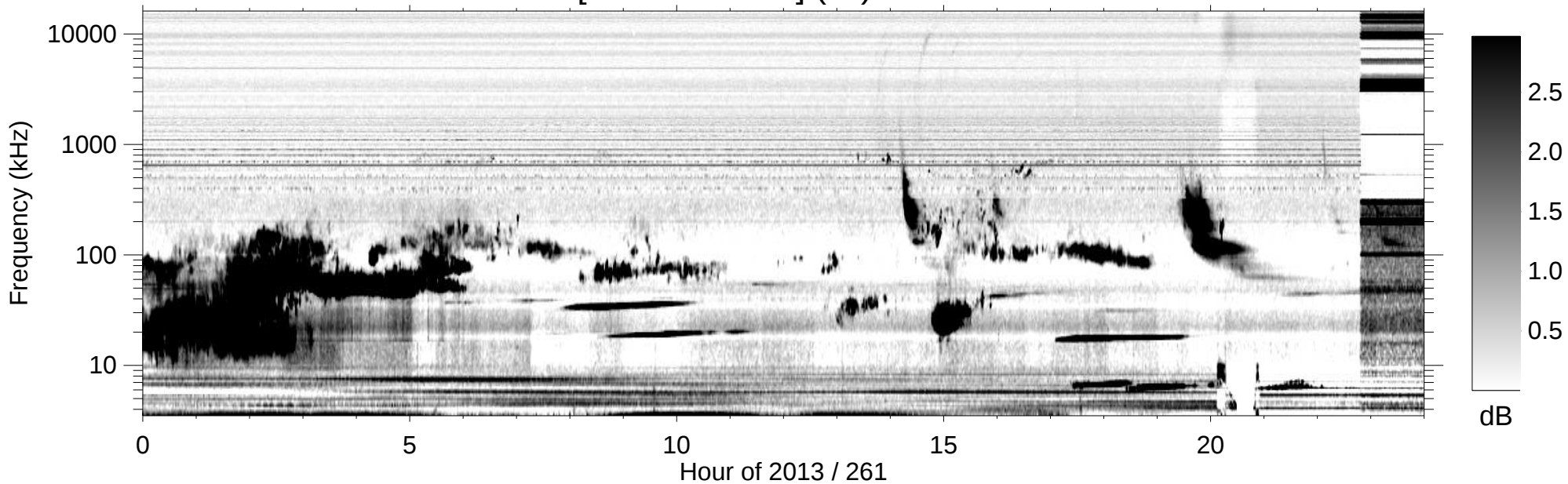
RPWS [ABCH1H2/Ex] (-B) 2013/09/18
