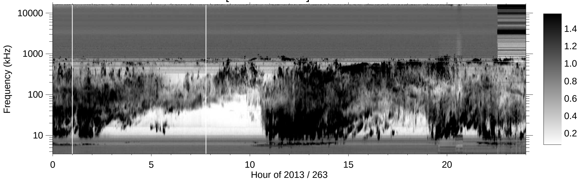
RPWS [ABCH1H2/Ex] (-B) 2013/09/20
