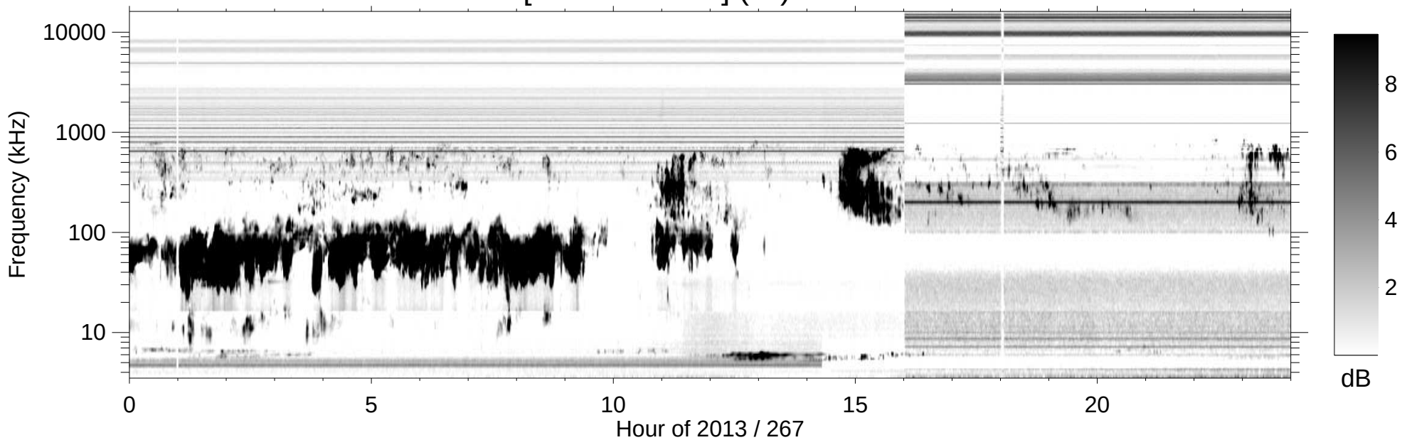
RPWS [ABCH1H2/Ex] (-B) 2013/09/24
