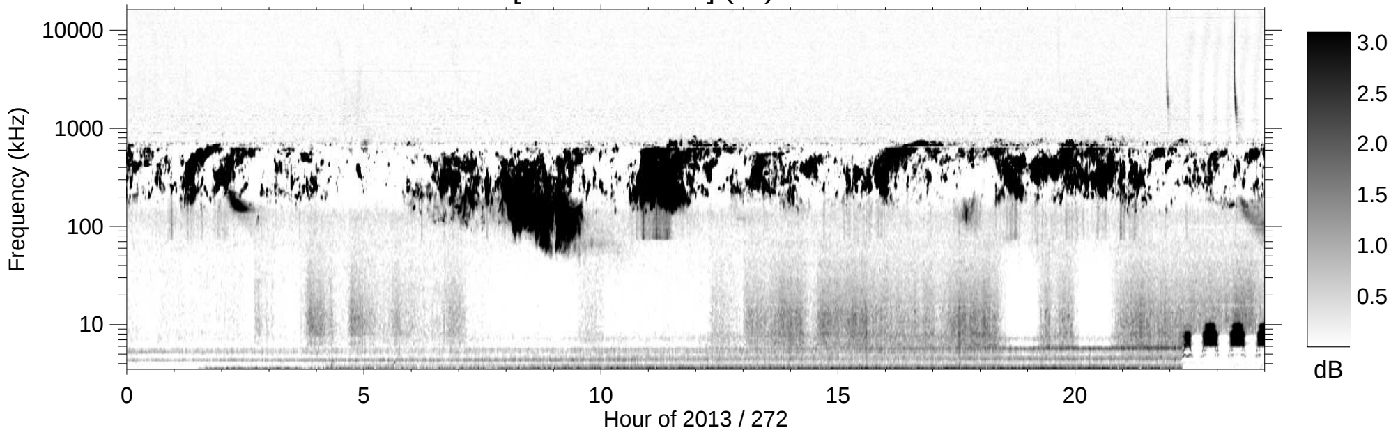
RPWS [ABCH1H2/Ex] (-B) 2013/09/29
