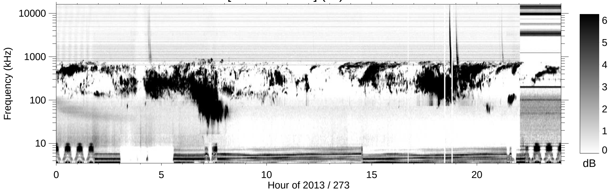
RPWS [ABCH1H2/Ex] (-B) 2013/09/30
