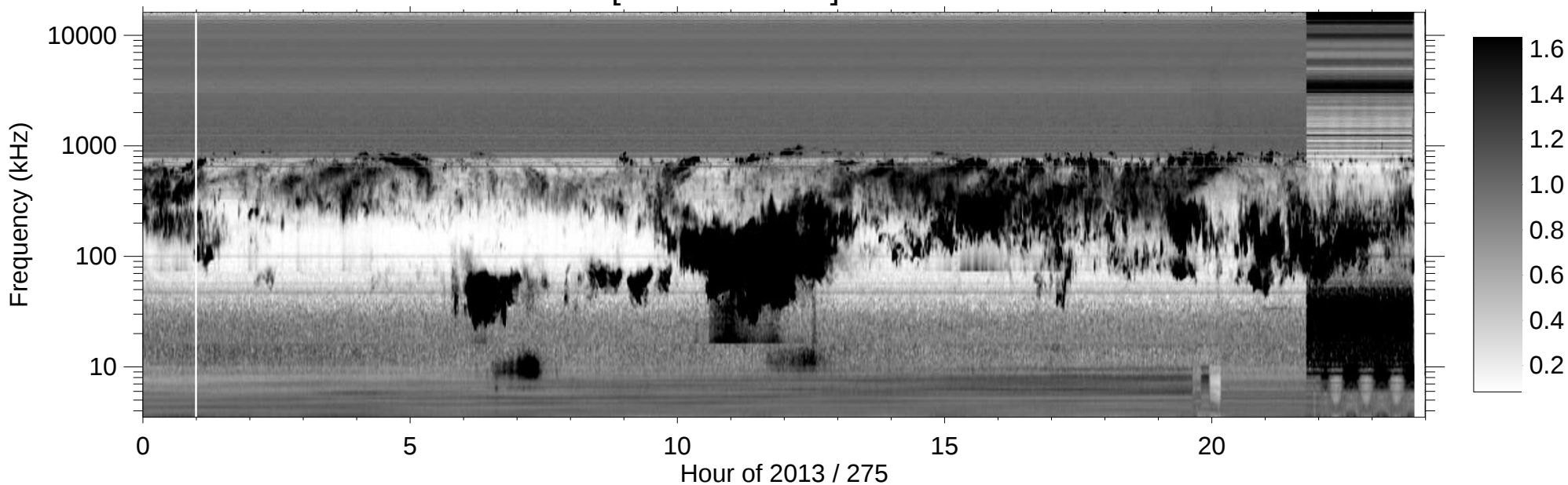
RPWS [ABCH1H2/Ex] (-B) 2013/10/02
