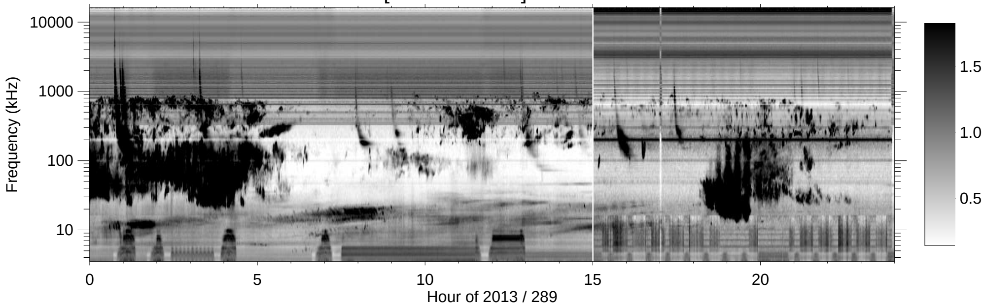
RPWS [ABCH1H2/Ex] (-B) 2013/10/16
